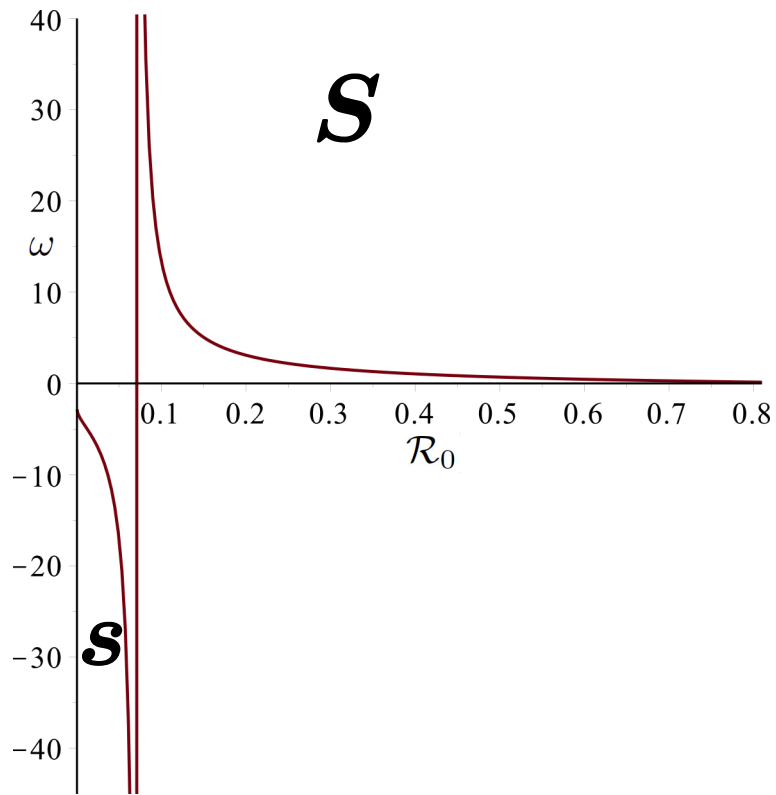
FIG. 4: Stability of wormhole supported by linear gas in terms of \omega and R_0 for a = 10 .
