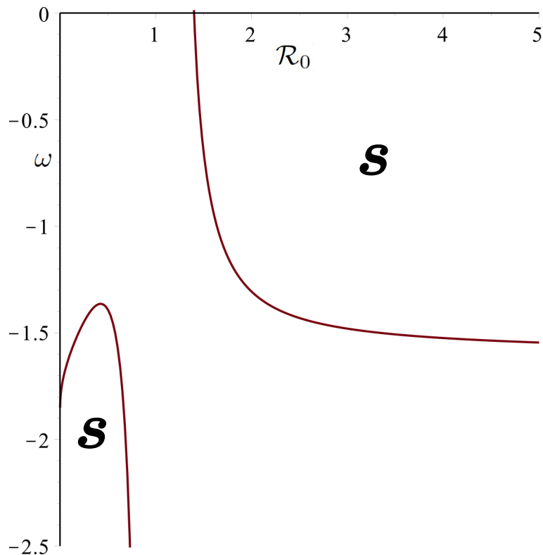
FIG. 2: Stability of wormhole supported by linear gas in terms of \omega and R_0 for a = 0.4 .
