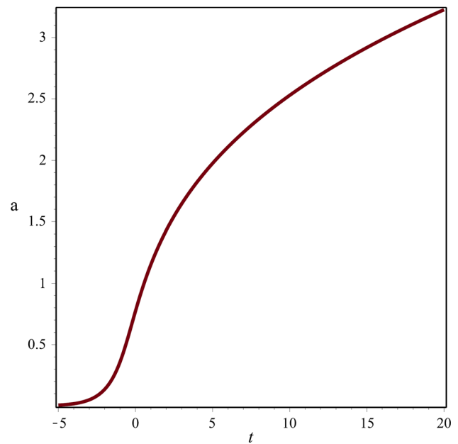
Fig. 2 Plot of the scale factor a versus the time t (for A = 1 and C = 1 )
