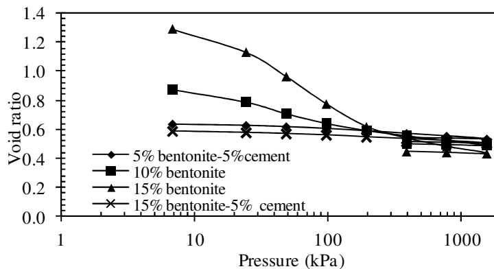
Figure 2. One dimensional free swell curves.
