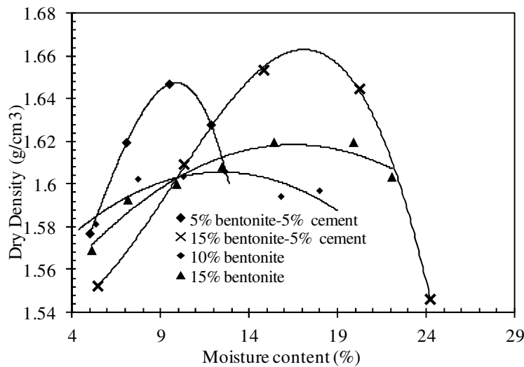
Figure 1. Compaction curves.
