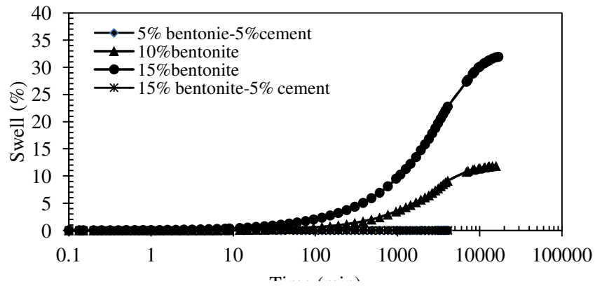
Figure 2. One dimensional free swell curves.
