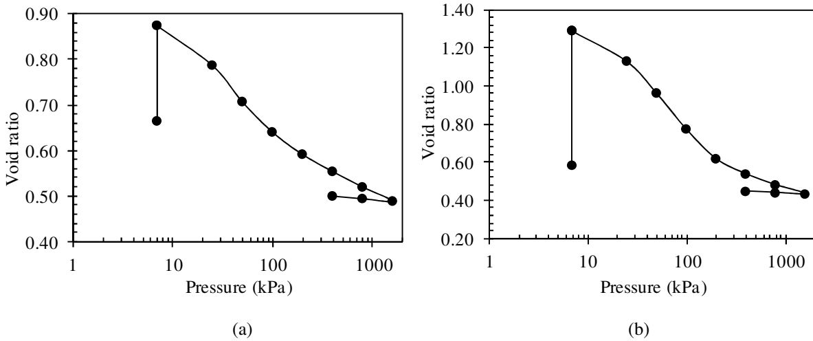
Figure 4. Consolidation curves of (a) 15% bentonite and, (b) 10% bentonite samples.
